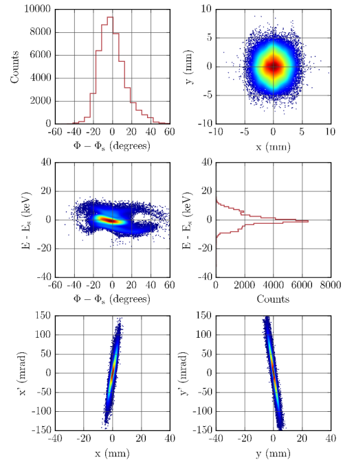
Figure 3: Phase Spaces of the RFQ output beam.
