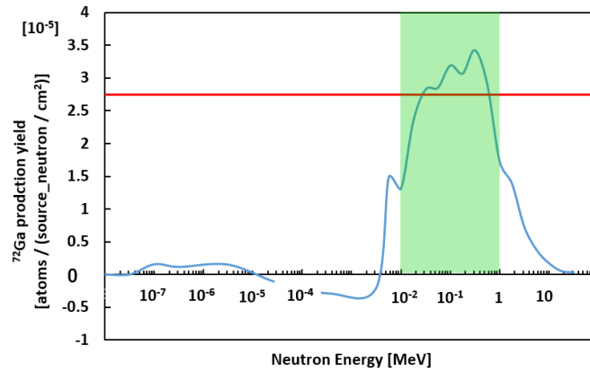
Fig. 4 Sensitivity of fast neutron detector.
