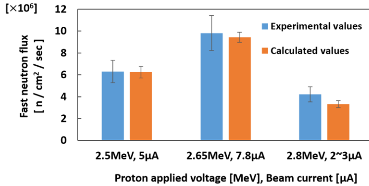
Fig. 7 Estimated fast neutron flux intensity.
