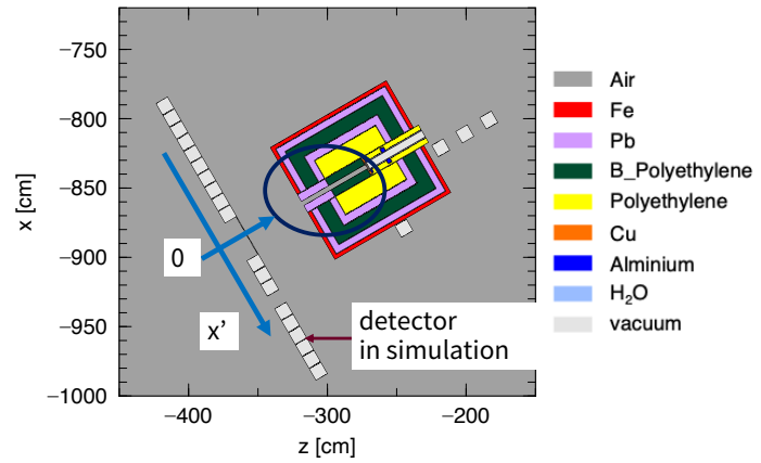
Figure 8: Target station with a BPE + Pb collimator.
