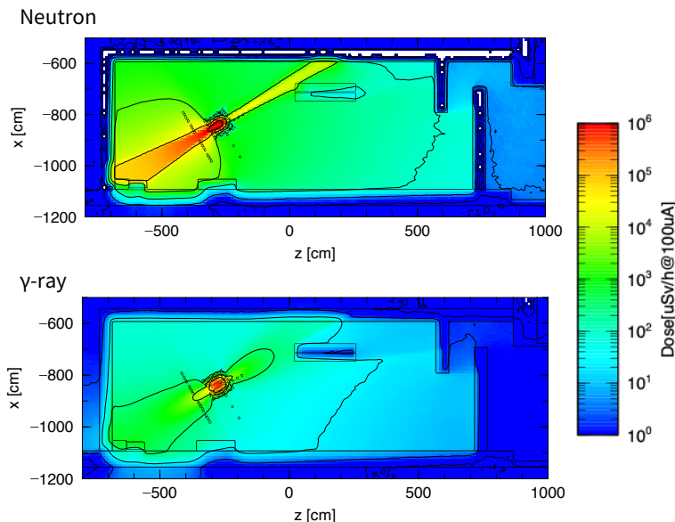
Figure 5: Dose rate distribution of neutrons and \gamma -rays at the RANS-II hall. The T-Track tally in PHITS is used. The mesh width for both x and z axis is 100 mm in the calculation.
