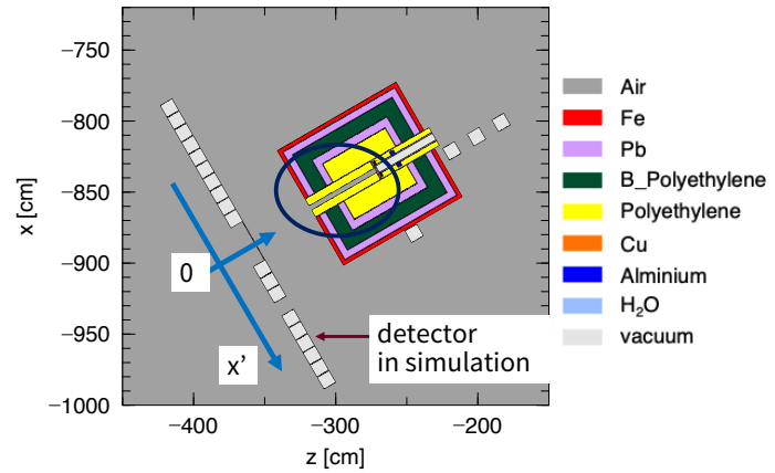
Figure 6: Target station with a PE collimator.
