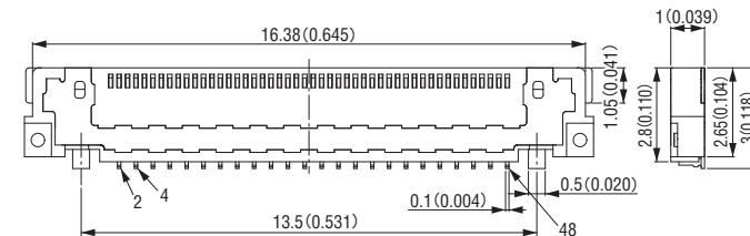
Surface mount base on a circuit board
