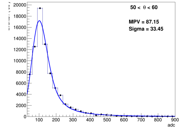
ADC distribution with a convolution function of Landau and Gau
