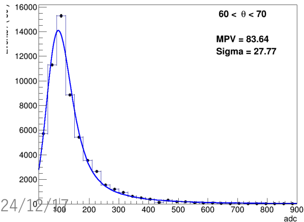
ADC distribution with a convolution function of Landau and Gau
