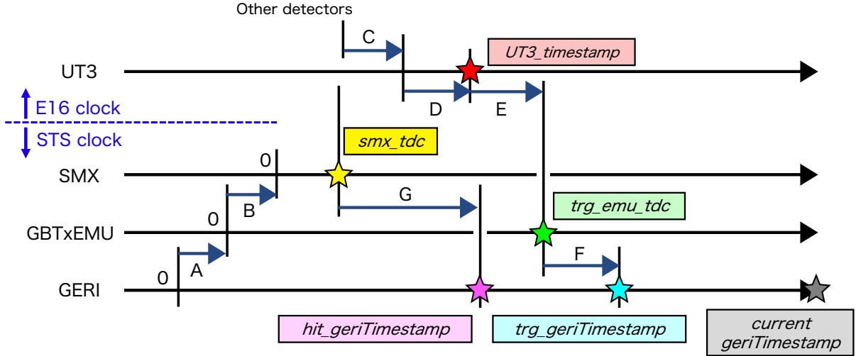
Figure D.1: Illustration of time axes and event timing in the STS readout system (reposted).
