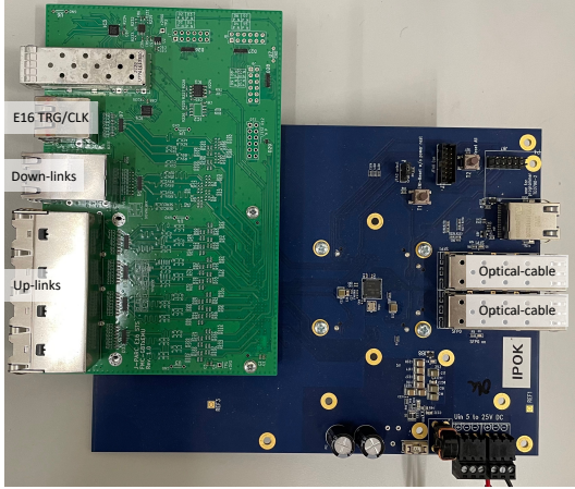
Figure 4.8: GBTxEMU and FMC board.
