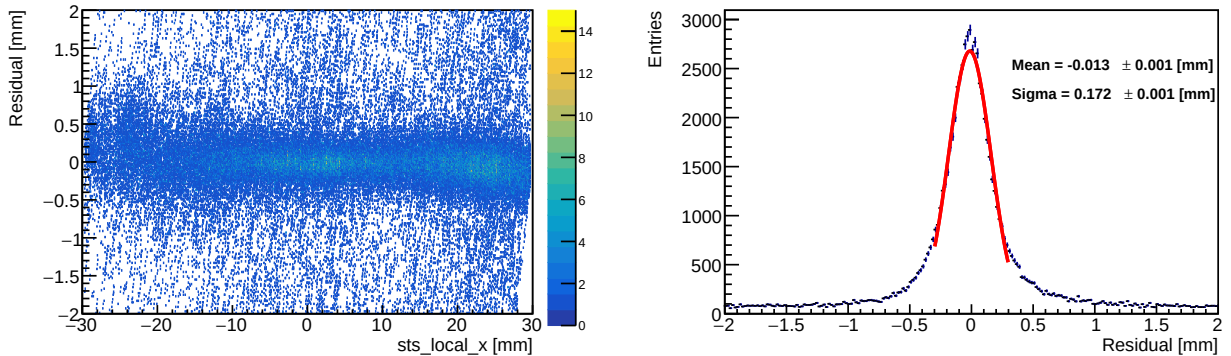
Figure 6.5: The 2D histogram with the horizontal axis as \text{sts\_local}_x and the vertical axis as the residuals (left) and the residual distribution over the entire \text{sts\_local}_x range of the 106 N-side (right).
