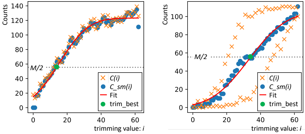
Figure C.6: Count values vs trimming values. The plot on the left shows an ASIC with a single S-curve, and the plot on the right shows an ASIC with two S-curves. The VDDM value of the ASIC on the right is relatively low.
