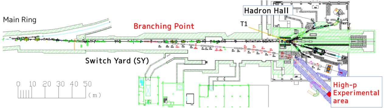
Figure 3.6: High-p beamline.
