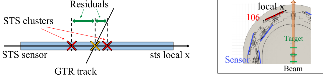
Figure 6.4: Definition of the residual between tracks and STS clusters (left) and the definition of \text{sts\_local}_x (right).
