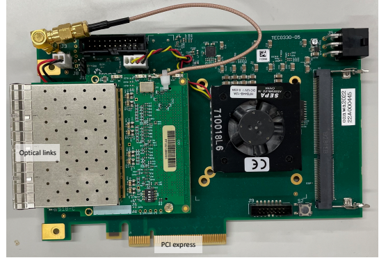
Figure 4.9: GERI board.
