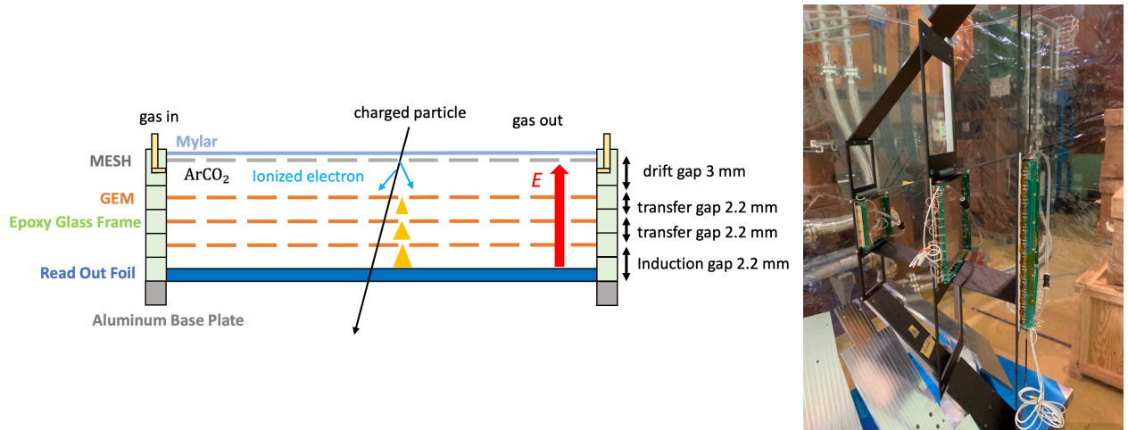
Figure 3.13: Conceptual diagram of GTR (left) and the CFRP frame and the provisionally mounted GTR are shown (right). The black frame is the CFRP frame, and from left to right on the middle tier are the GTR100, GTR200, and GTR300 [36].
