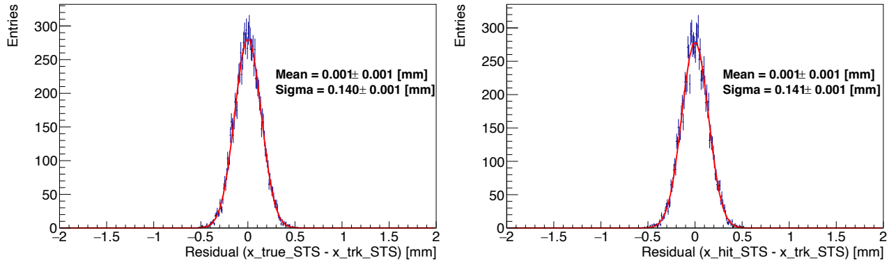
Figure 6.10: Residual distributions between the STS intersection of the track reconstructed using only the three GTR layers and the true STS incident position (left), and between the STS intersection and the detected STS position (right) from the Monte Carlo simulation.
