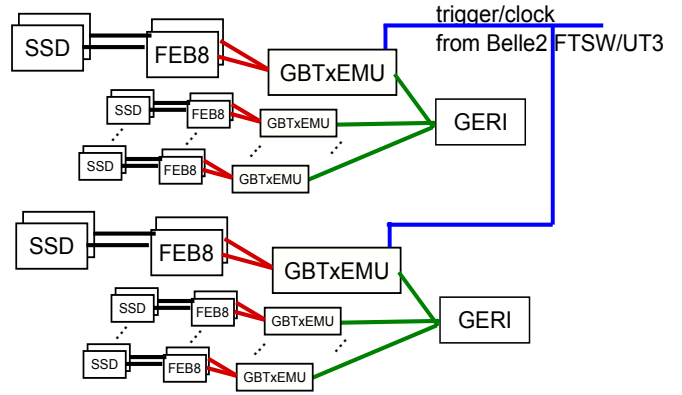
Figure 4.11: E16 STS readout chain.
