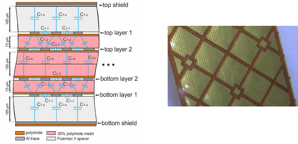
Figure 2.6: Cross section of a stack of readout microcables [19] (left) and photo of microcables (right). The diagram illustrates the effective capacitances between the different cable layers.
