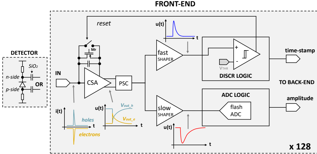
Figure 2.8: SMX circuit [25].
