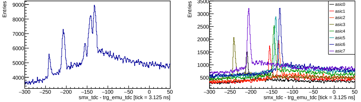
Figure 6.13: Timing distribution in smx_tdc misalignment (104 N-side).
