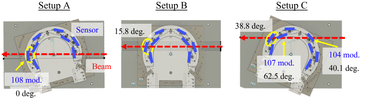
Figure 5.5: Top view of each setup.
