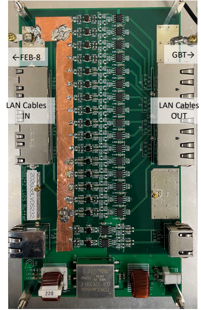
Figure 4.7: LVDS Repeater.
