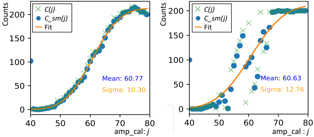
Figure C.7: Pscan of the FAST thresholds performed with trim_best set. The plot on the left shows an ASIC with a single S-curve, and the plot on the right shows an ASIC with two S-curves. The VDDM value of the ASIC on the right is relatively low.
