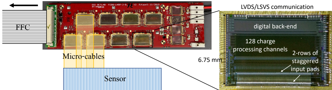
Figure 2.7: FEB-8 (left) and STS-MUCH XYTERv2 (right) [25].
