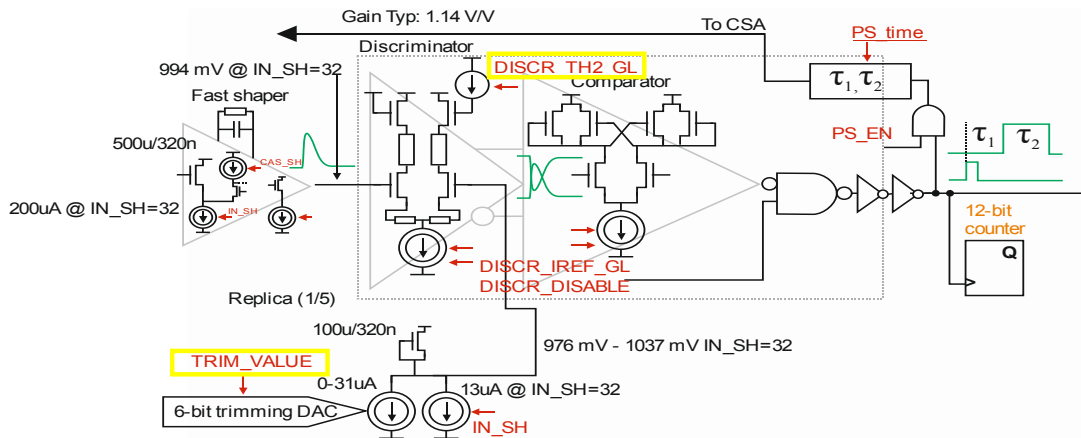
Figure C.5: FAST discriminator [25].
