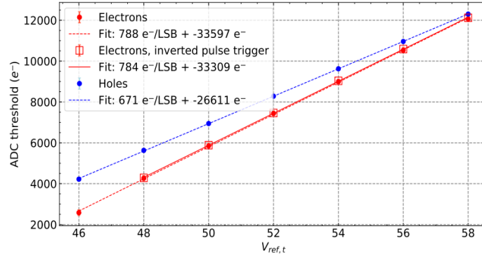
Figure C.4: The relationship between V_{\text{ref\_T}} and the ADC lowest threshold. The slope is slightly different on the N-side (electrons) and P-side (holes).
