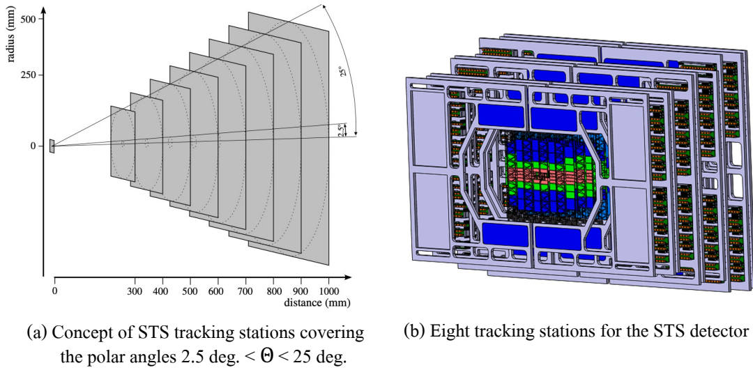
Figure 2.13: CBM STS layout [18, 19].
