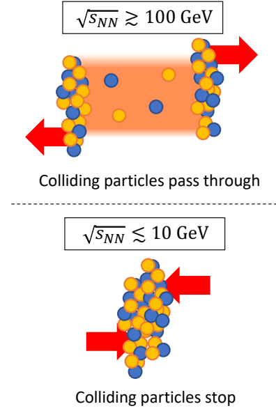
Figure 1.3: Differences in Collisions Depending on \sqrt{s_{NN}} [11].
