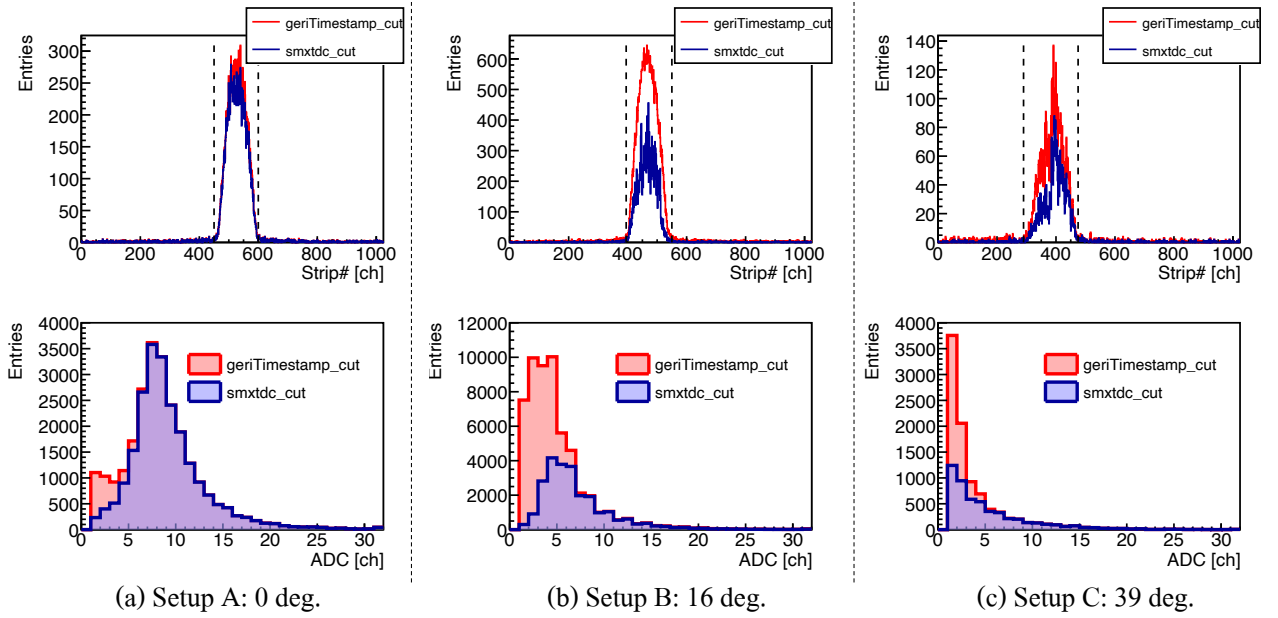
Figure 5.17: The hit profiles (upper) and ADC distributions (lower) for the geriTimestamp cut (red) and smxtdc cut (blue) in each setup.
