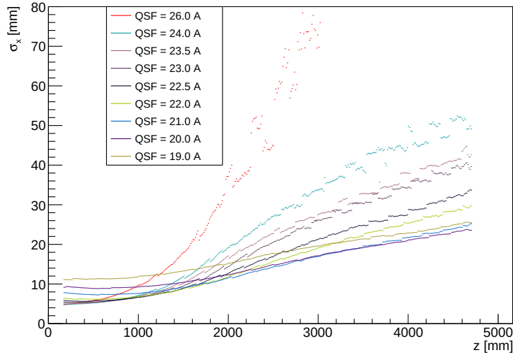
Figure 5.3: The z -dependence of the beam profile. Using a magnet setting of AR = 5.0 \text{ GeV} and p = 3.0 \text{ GeV} , the current of the QSF magnet was varied while tracking hit information from two jet chambers. The hit map was projected onto the x -axes, and the resulting \sigma values were obtained by fitting the distributions with a Gaussian function. z=0 is the extraction point [47].
