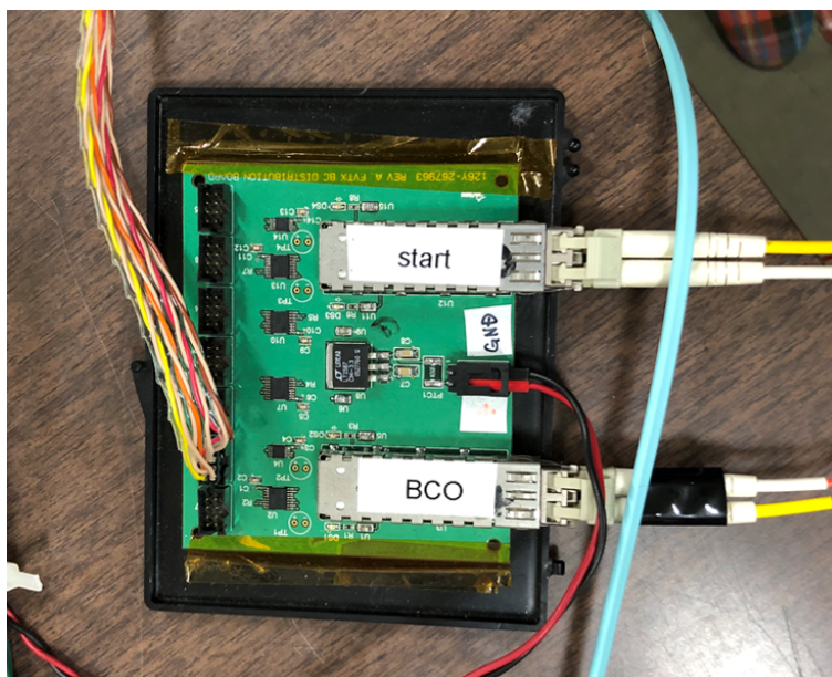
図 2.14 Beam Clock Distribution Board
